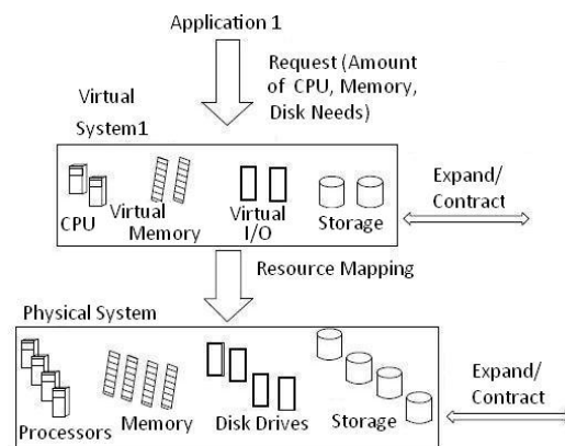
Fig-1 mapping of virtual to physical resources
