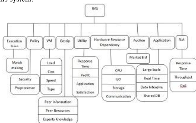
Fig. 2 Cloud Computing Resource Allocation Strategies.
