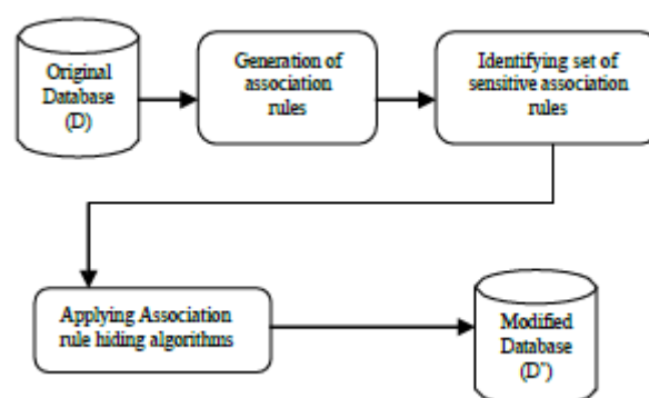
Figure 2: Framework for Hiding Sensitive Association Rules
